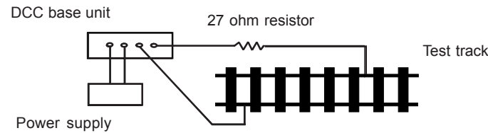
Figure 3. Diagram of test track
