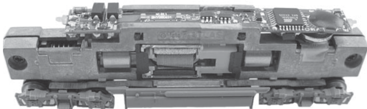
Figure 2. shows how to install 0001812 decoder
