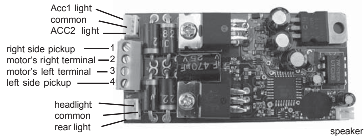
Figure 2. 0001818 decoder wiring diagram
